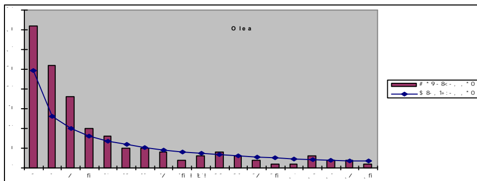
diameter distribution for the Yemerahene-Kerstos church
