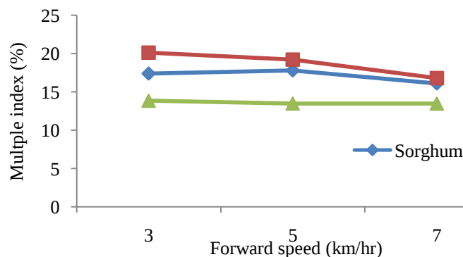
Figure 3. Effects of planter forward speeds on seeds multiple indices
